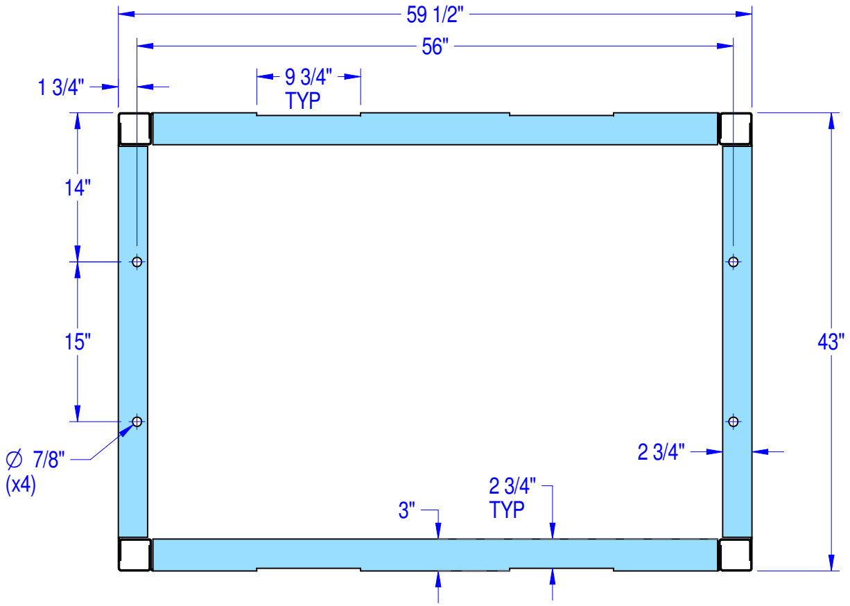
Oven's Contact Area with Floor
